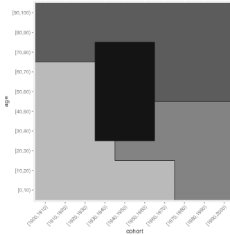
(c) Piecewise constant true hazard – heatmap
