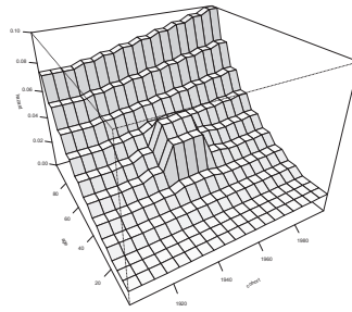
(b) Smooth true hazard – perspective
