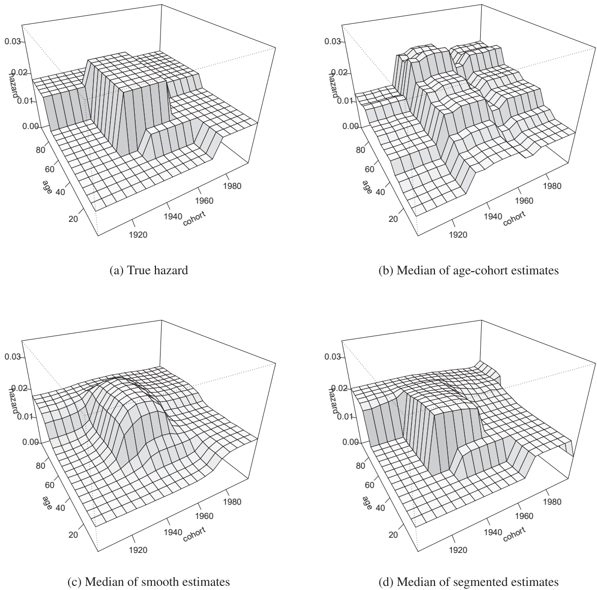
Figure 4: Piecewise constant true hazard and corresponding estimates. The sample size is 4000 and the hazard estimates are medians taken over 500 simulations. The estimations are performed in the age-cohort plane and with different methods. Panel (a) represents the true hazard used to generate the data, panel (b) represents the hazard estimated using the age-cohort model, panel (c) represents the smoothed estimate, and panel (d) represents the segmented estimate with the EBIC criterion.
