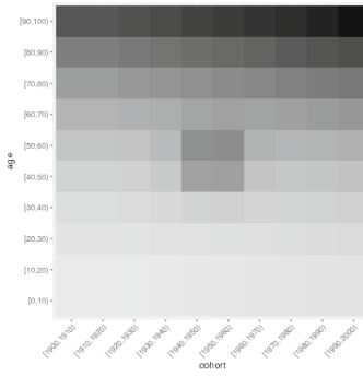
(a) Smooth true hazard – heatmap
