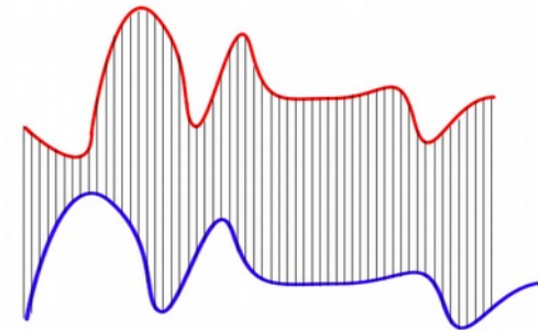
Euclidean Matching
