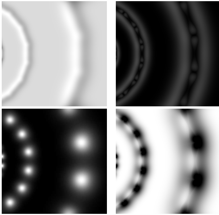
Figure 4: Functions \sum_{k \in \frac{\mathbb{Z}}{N\mathbb{Z}}} |\widehat{\psi}(2^j R^k \cdot)|^2, \Phi_2, \Phi_3 and \Phi_4 + \sum_{\gamma \in \Gamma^*} |\widehat{\psi}(2^j R^k \cdot)|^2 - \Phi_1 - \Phi_2 - \Phi_3 for \psi as in (2) and N = 9 . Only restrictions to the domain [\pi/2, 5\pi/2] \times [-\pi, \pi] are shown.
