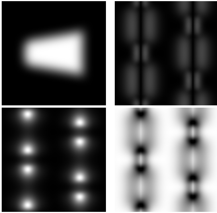
Figure 3: Functions |\widehat{\psi}_a|, \Psi_1, \Psi_3 and \Psi_4 + \sum_{\gamma \in \Gamma^*} |\widehat{\psi}(\cdot + \gamma)|^2 - \Psi_1 - \Psi_2 - \Psi_3 for \psi as in (2) and N = 9 . Only restrictions to the domain [\pi/2, 5\pi/2] \times [-\pi, \pi] are shown.
