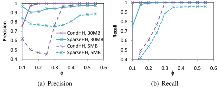
Fig. 7. Accuracy as \phi varies on Worldcup data
