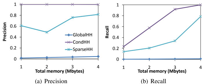
Fig. 11. Accuracy on Taxicab data as memory varies
