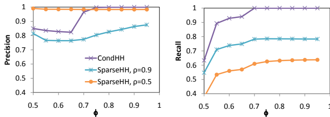
Fig. 12. Accuracy as \phi varies on Taxis data
