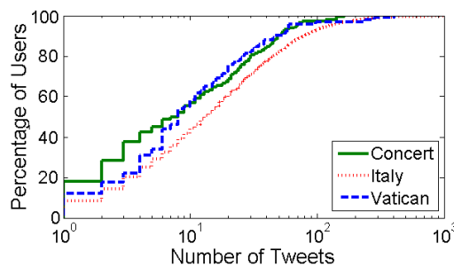
Fig. 5: CDF: Comparison of Number of Tweets
