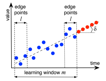
Fig. 2. Derivative-based Prediction.
