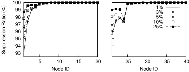
(a) Relative error \epsilon^{rel} ( \epsilon^{abs} = 25 , \epsilon_T = 0 ).
