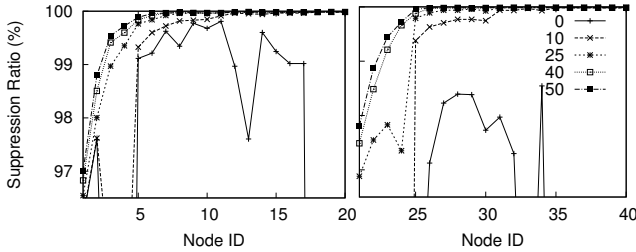
(b) Absolute error \epsilon^{abs} ( \epsilon^{rel} = 5\% , \epsilon_T = 0 ).
