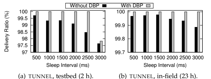
Fig. 11. Delivery ratio for the TUNNEL dataset.
