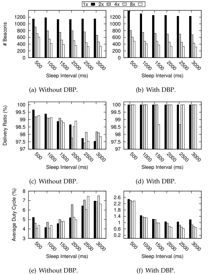
Fig. 15. TUNNEL, testbed (4 h): beacon transmissions, delivery ratio, and duty cycle for different combinations of sleep intervals and beacon intervals. Note the different scale in the bottom charts for duty cycle.
