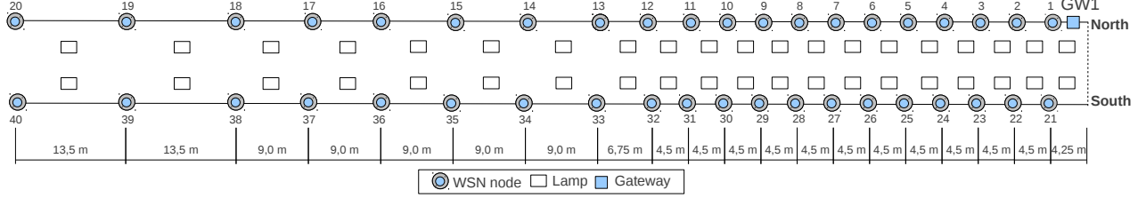
Fig. 3. Physical placement of WSN nodes in TUNNEL.
