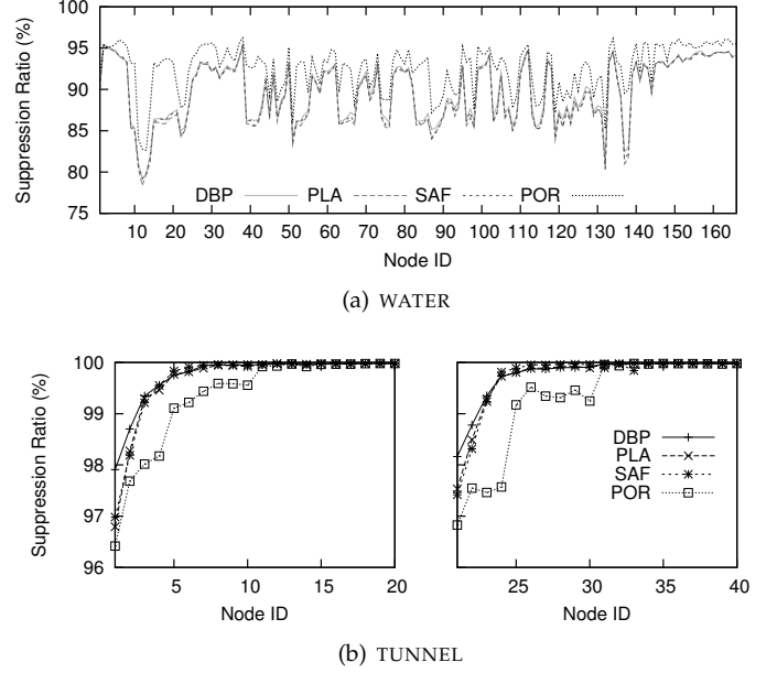
Fig. 4. DBP vs. state-of-the-art techniques on individual nodes in WATER and TUNNEL.
