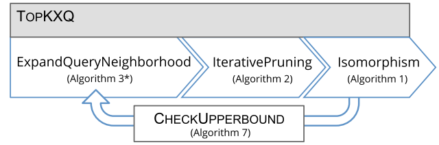
Fig. 7 A visualization of the TOPKXQ algorithm
